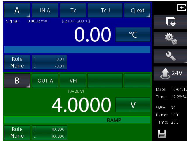
Figure 60 – Ramp function active
