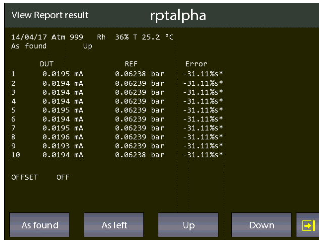
Figure 82 – Display Report results
